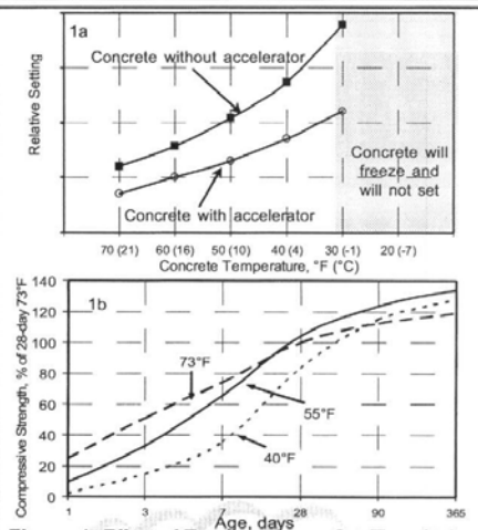
Figure 1 Effect of Temperature on Set Time (1a) and Strength (1b) of Concrete
